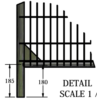
DETAIL P SCALE 1 / 8
