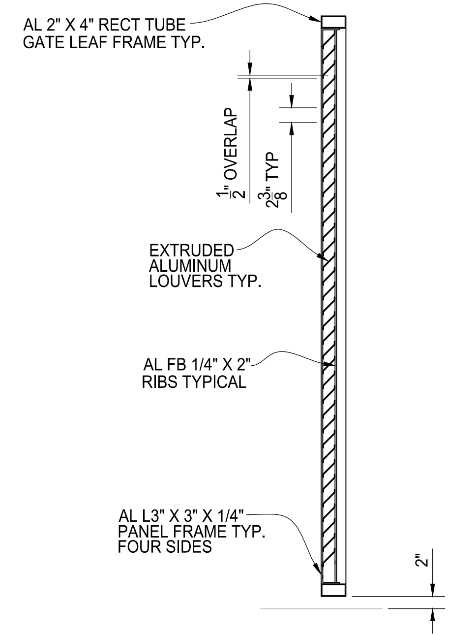
B TYPICAL GATE SECTION
