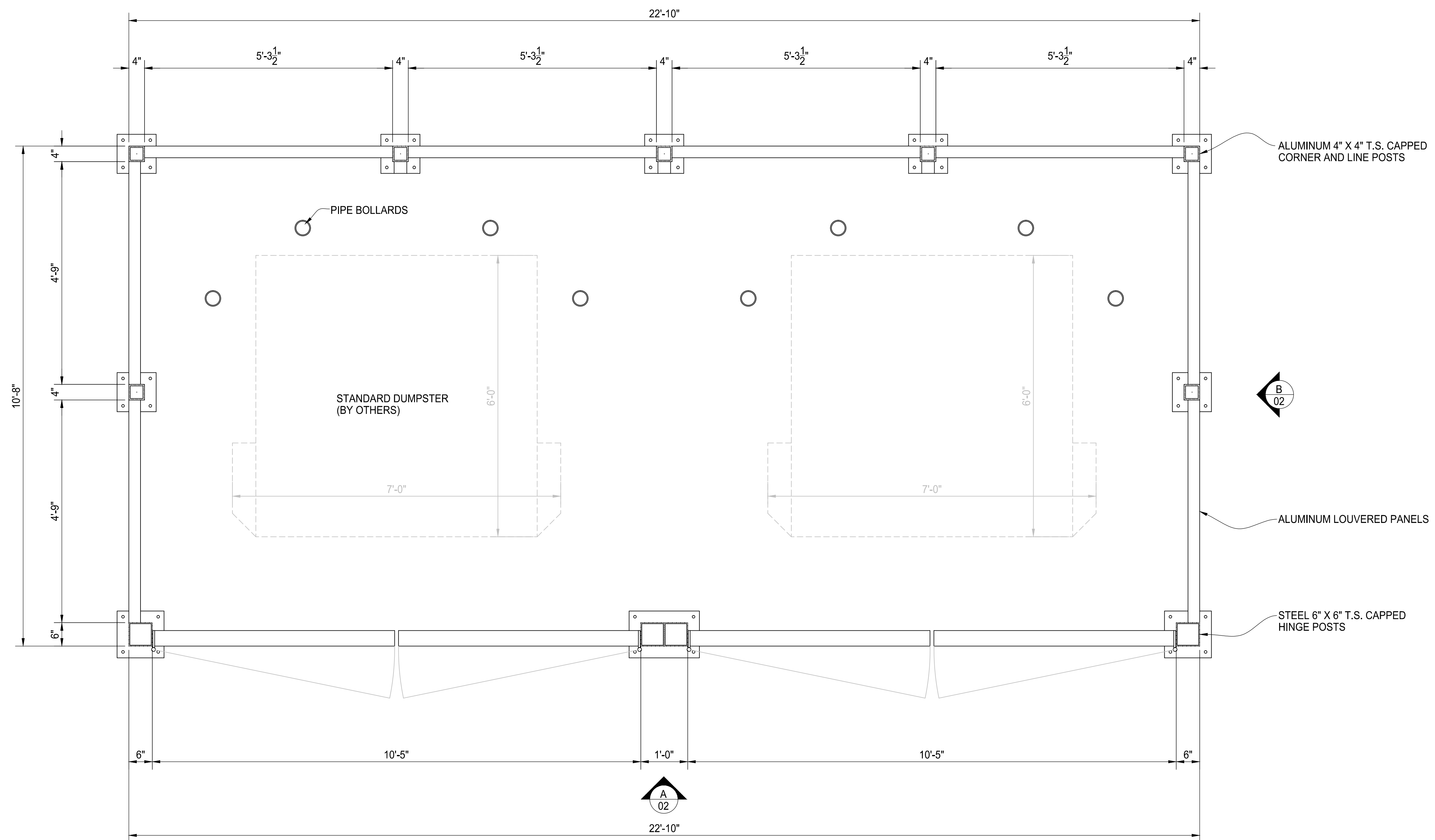
PLAN VIEW @ DUMPSTER ENCLOSURE
